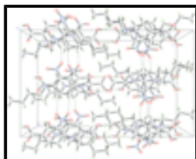
Fig. 2. The crystal packing of the title compound, viewed along the a axis. Dashed lines indicate the hydrogen bonding.
